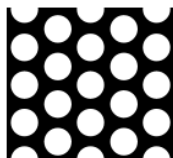
5/32" @7/32" STAGGERED 46%
