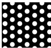
3/32" @5/32" STAGGERED 32%
