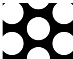
7/16" @9/16" STAGGERED 51%
